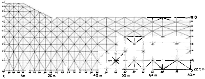
FIG. 7. Finite-Element Discretization of Embankment and Subsols for CRISP Analysis
