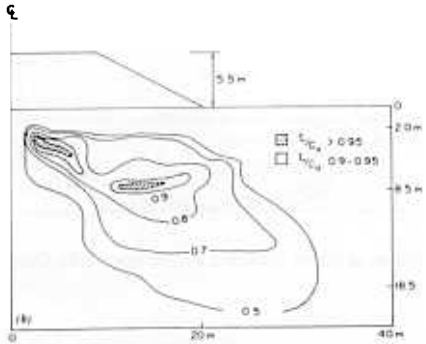
FIG. 16. Contour Plots of Normalized Shear-Stress Ratios
